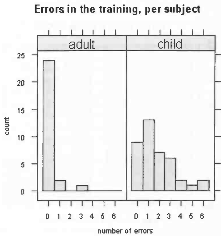
Figure 5.2: Histogram showing the number of errors per subject (prediction errors and rationality errors taken together) for the last six items of the training.
