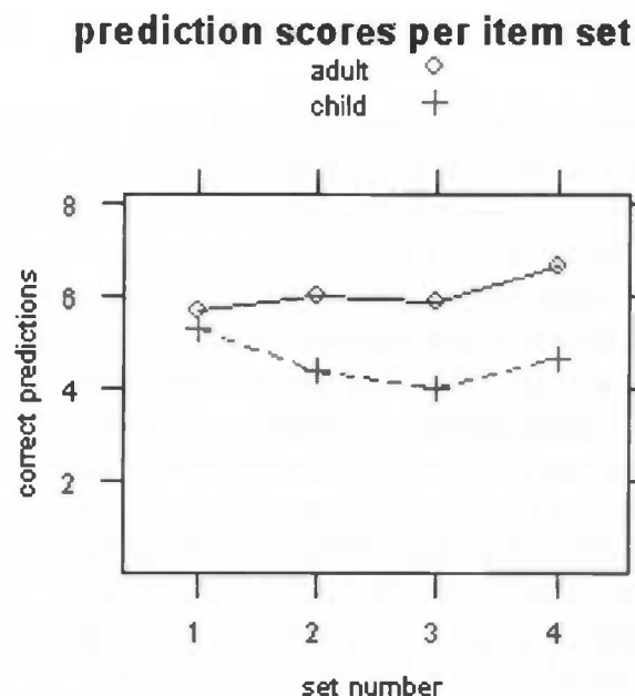
Figure 5.4: Average prediction scores per set. The upper line represents the adults, the lower line represents the children.
