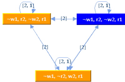
Figure 4. Counter-model to Heloise knowing the color of her own hat in the initial situation of the ‘wise persons’ puzzle. The counter-model to Abelard knowing the color of his hat is almost identical, except that the relations between the worlds are for agent 1 (Abelard), not agent 2 (Heloise).
